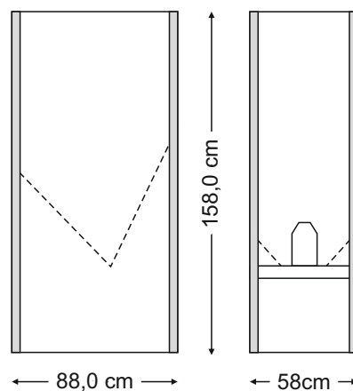
320kg pelletbunker
