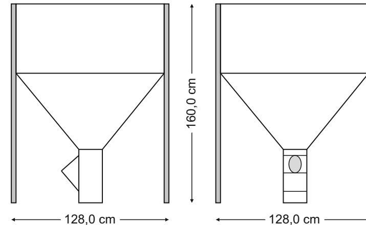
500kg pelletbunker
